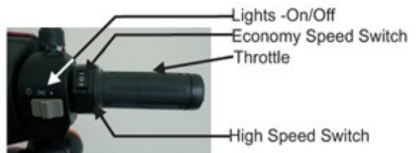
Right Handlebar
